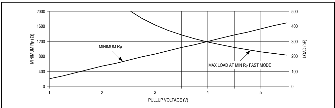
Figure 11. I²C Fast Mode Pullup Resistor Selection Chart
