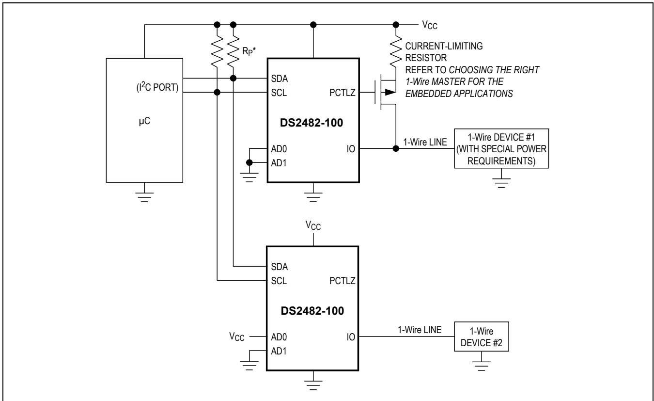
Figure 10. Application Schematic
