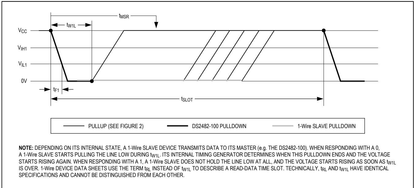
Figure 6. Write-One and Read-Data Time Slot
