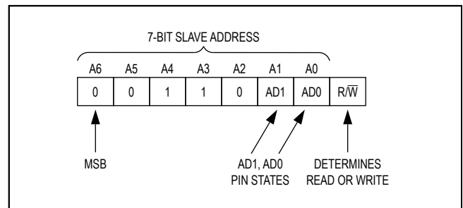
Figure 8. DS2482-100 Slave Address
