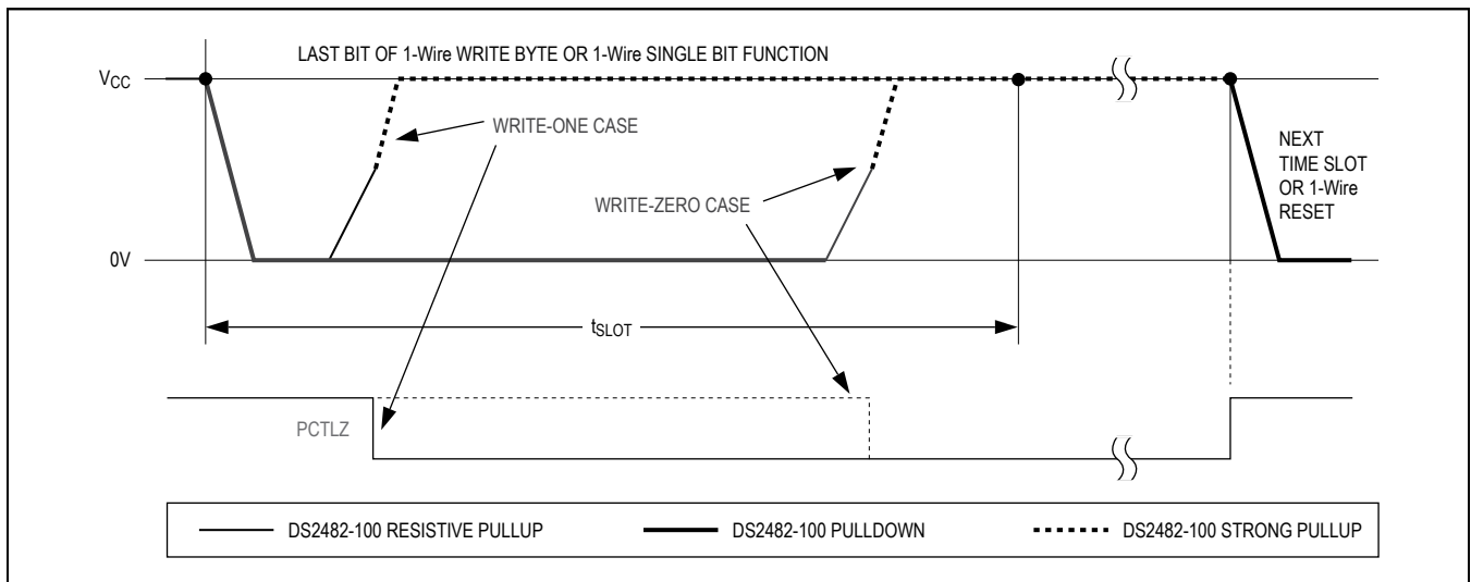
Figure 3. Low-Impedance Pullup Timing
