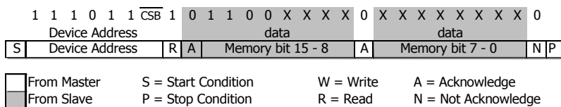
Figure 12: I 2 C answer from MS5611-01BA
